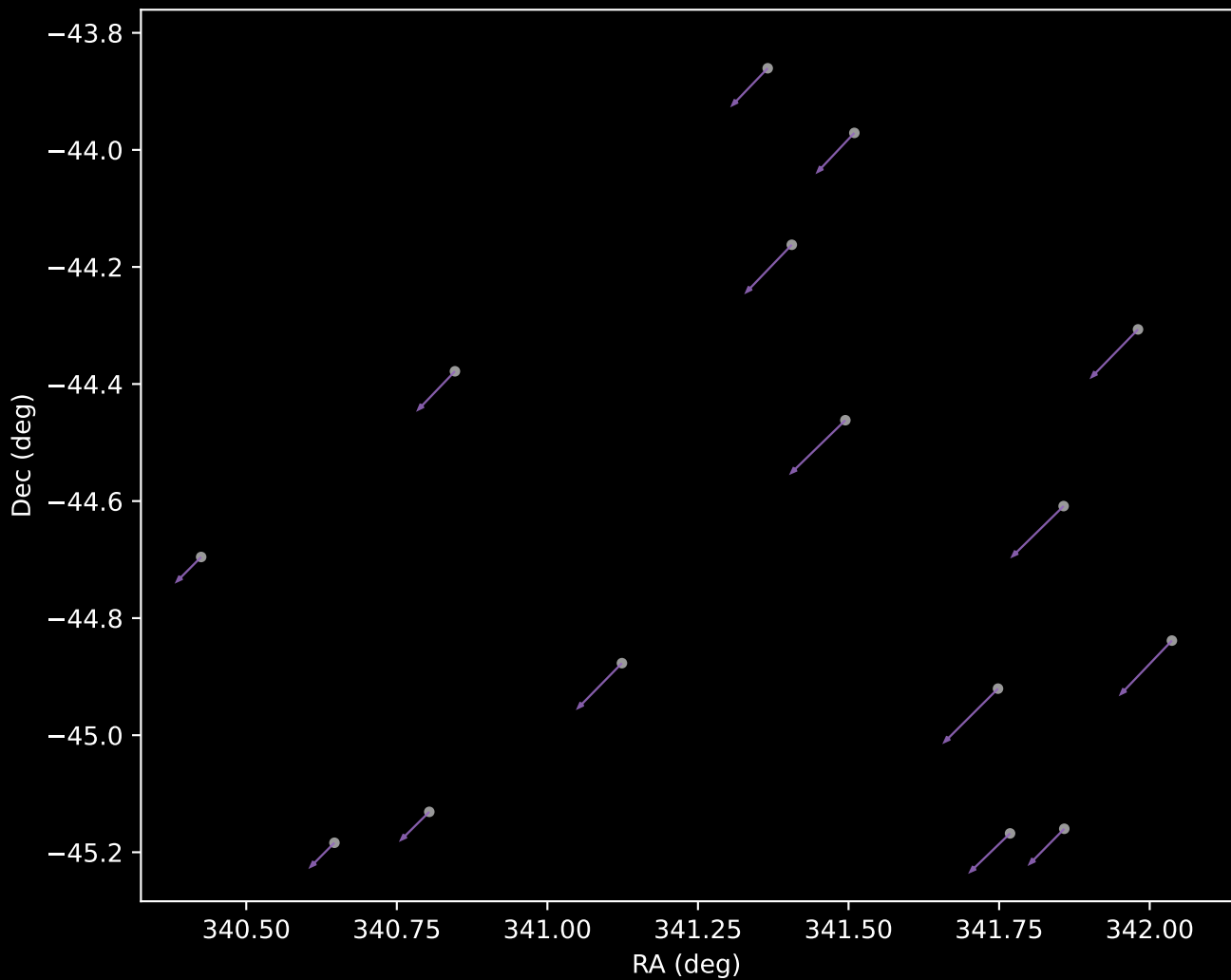
APOGEE DR17 Cluster 28 Proper Motion Vectors (n=15)
