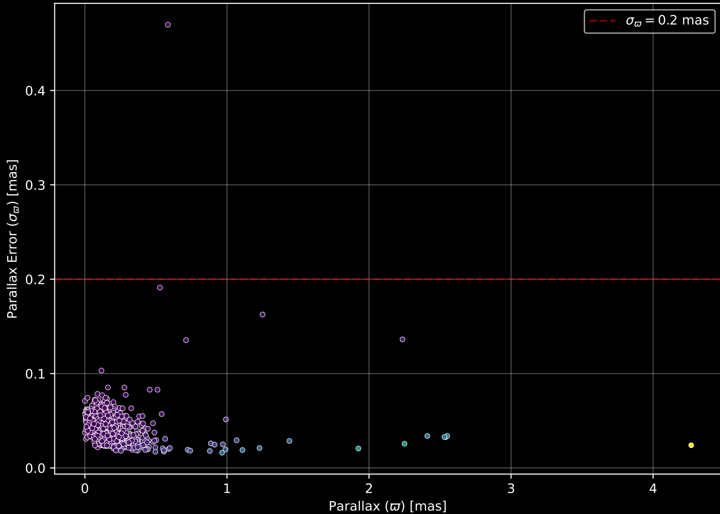
APOGEE DR17 Field: [335+06] Parallax Quality (n= 587)
