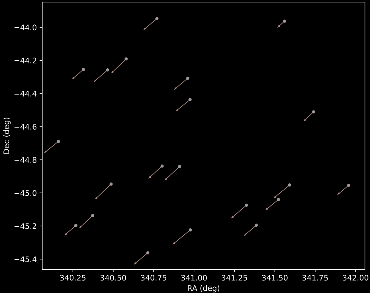
APOGEE DR17 Cluster 11 Proper Motion Vectors (n=21)
