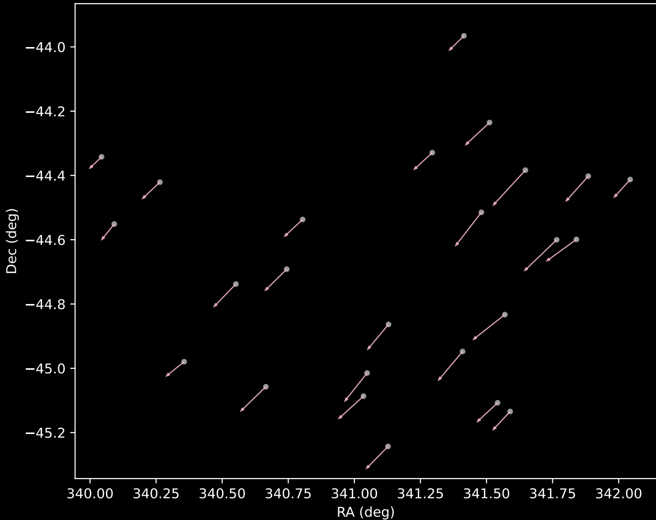
APOGEE DR17 Cluster 13 Proper Motion Vectors (n=25)
