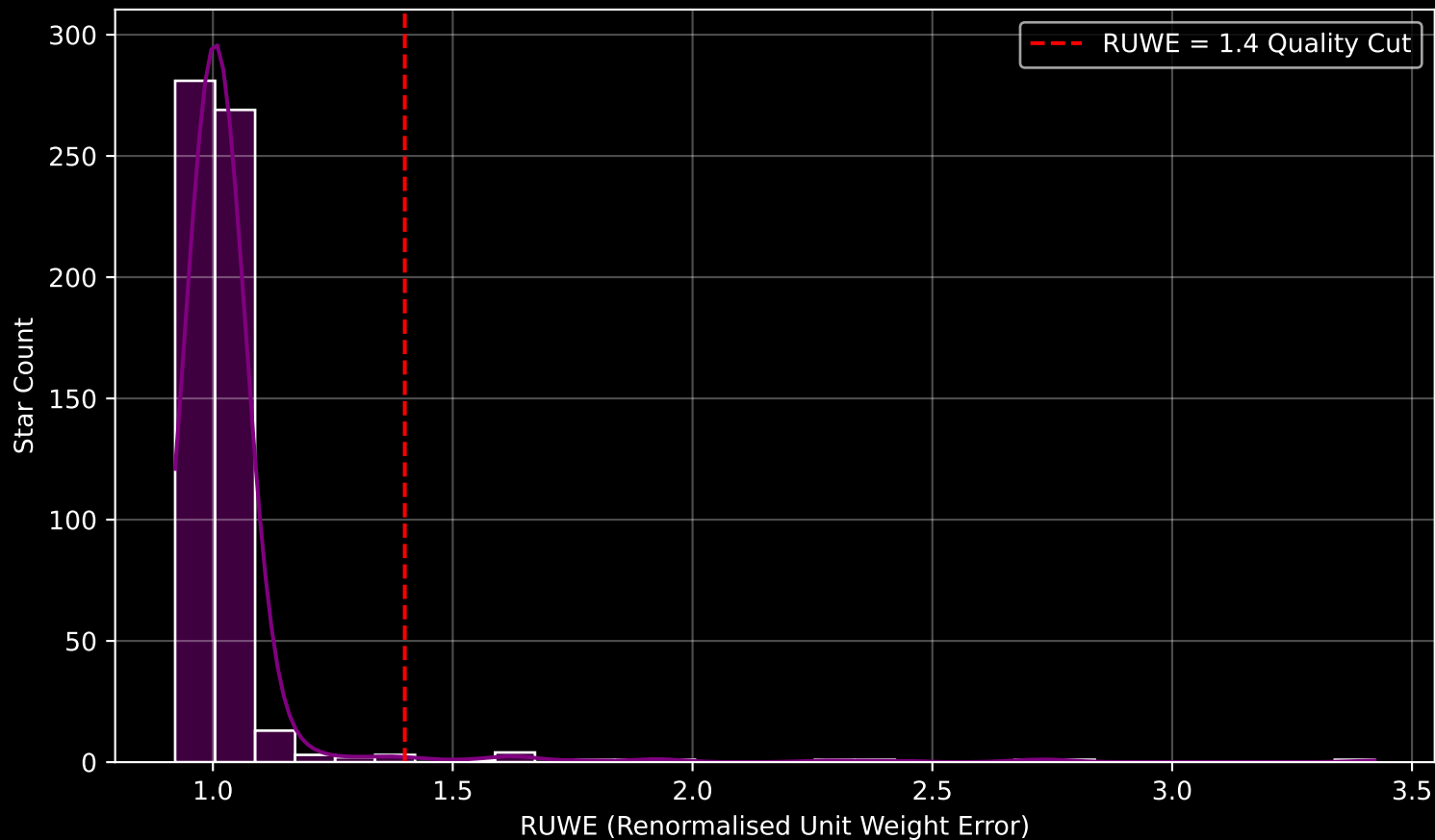
GAPOGEE DR17 Field [335+06] RUWE Distribution (n= 584)
