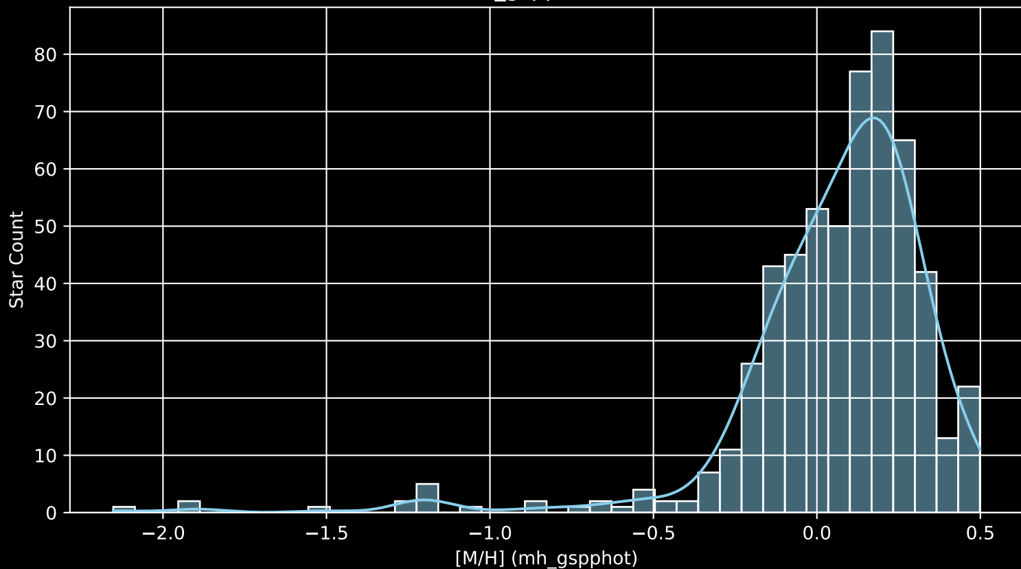
APOGEE DR17 Field: [335+06 [M/H] (mh_gspphot) (n= 564)
