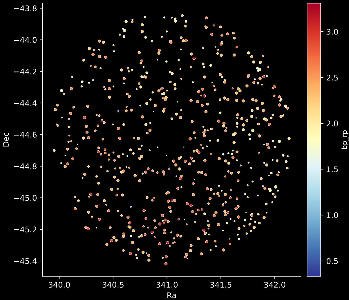
APOGEE DR17 Field: [335+06] Stars: 587
