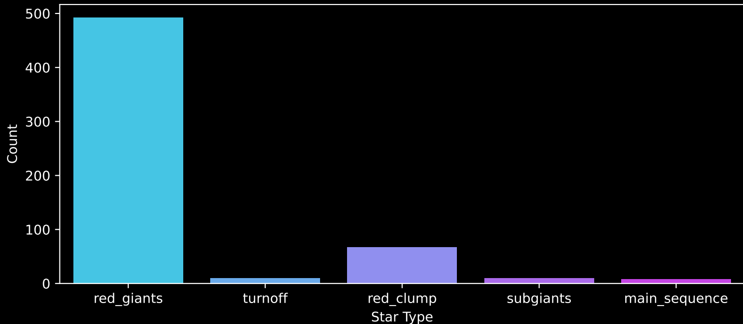
APOGEE DR17 Field: [335+06] Count plot of Star Type
