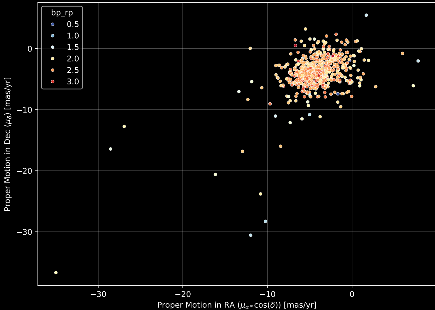
APOGEE DR17 Field: [335+06] Proper Motion Diagram (n= 587)
