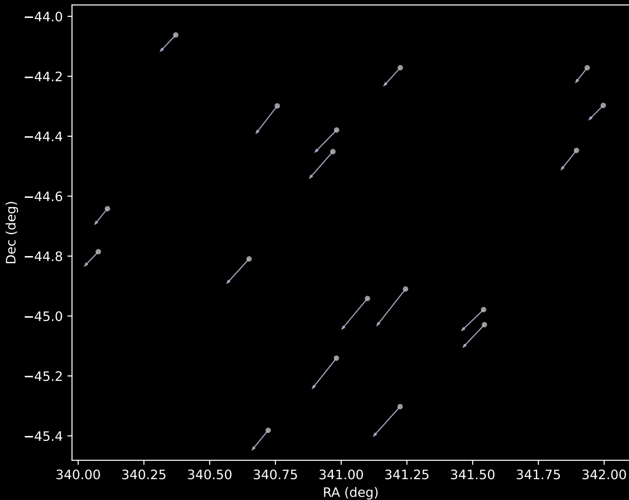
APOGEE DR17 Cluster 29 Proper Motion Vectors (n=18)
